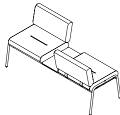
DOUBLE BENCH MIT ABLAGE MITTIG | WITH MIDDLE TRAY (FACE-TO-FACE) 1.675 x 704 x 783 mm
