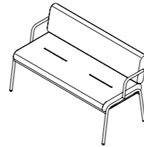
DOUBLE BENCH 1.350 x 655 x 783 mm
