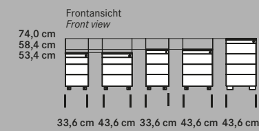
WINEA MAXX Container WINEA MAXX pedestals
