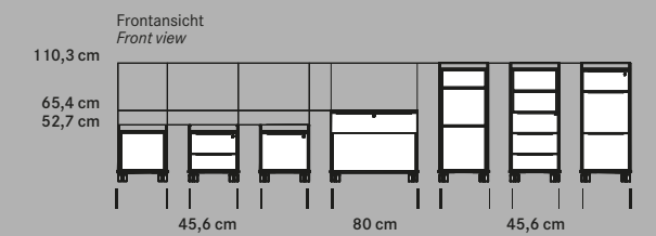
WINEA MAXX Caddy WINEA MAXX caddy
