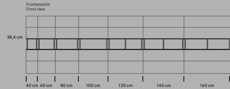
WINEA MAXX offene Mittelregale WINEA MAXX open intermediate shelves
