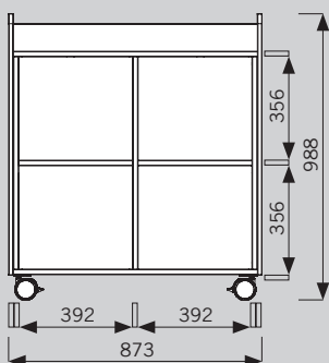
LARGE offen
