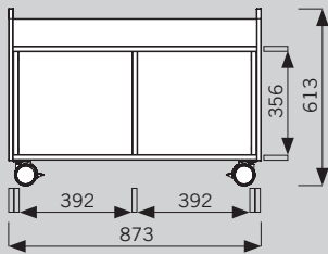
SMALL offen
