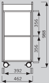
MEDIUM offen
